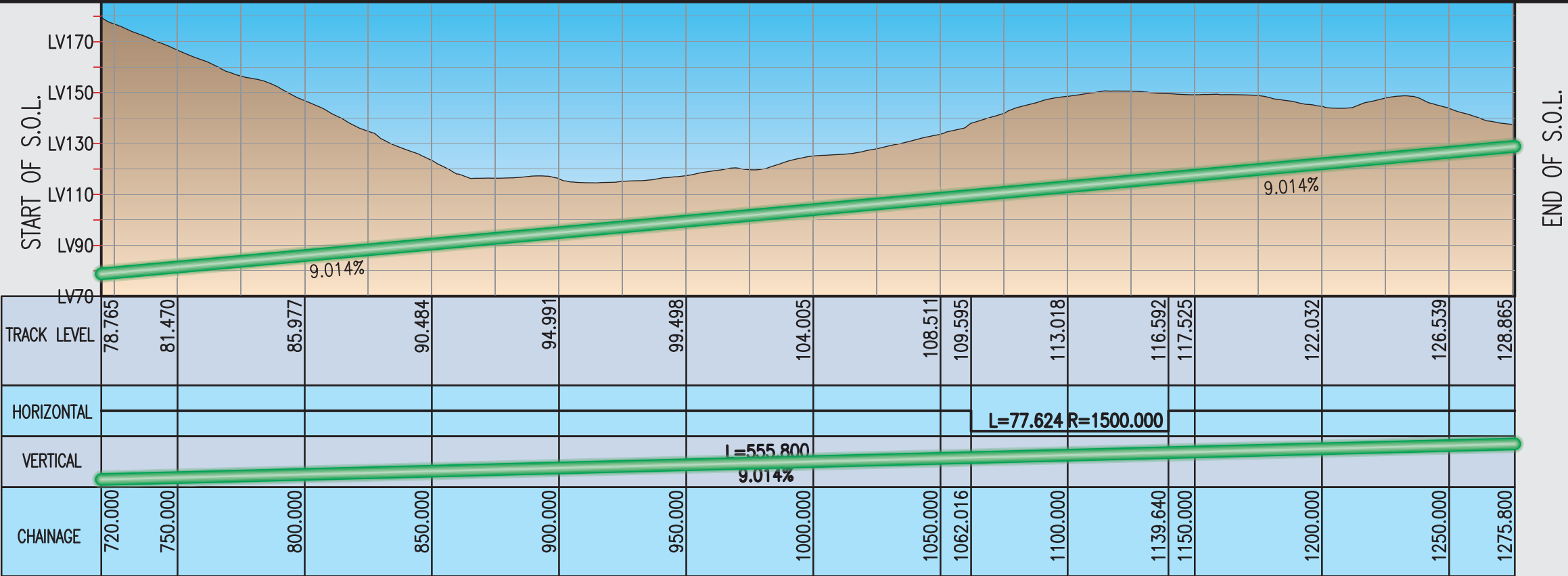
VERTICAL PROFILE ALONG TUNNEL HORI SCALE 1:2000 VERT SCALE 1:2000
