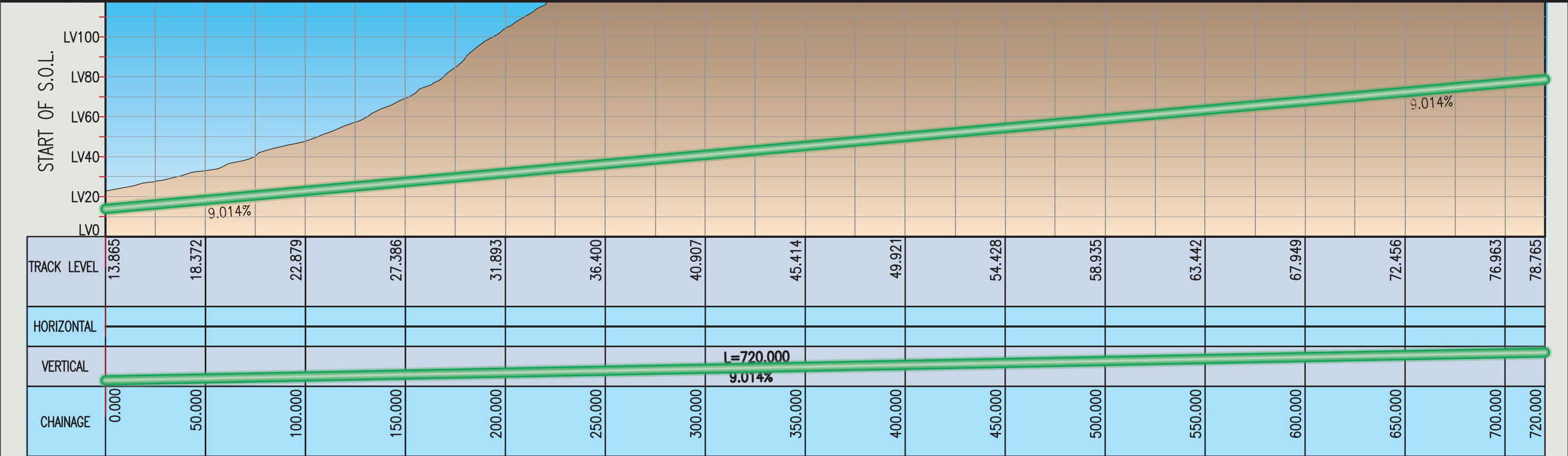
VERTICAL PROFILE ALONG TUNNEL
